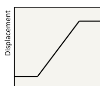
Pilot Pressure Positive Flow Control, Hydraulic Pilot
