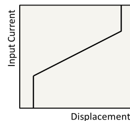
Proportional Control, Electric (positive)
